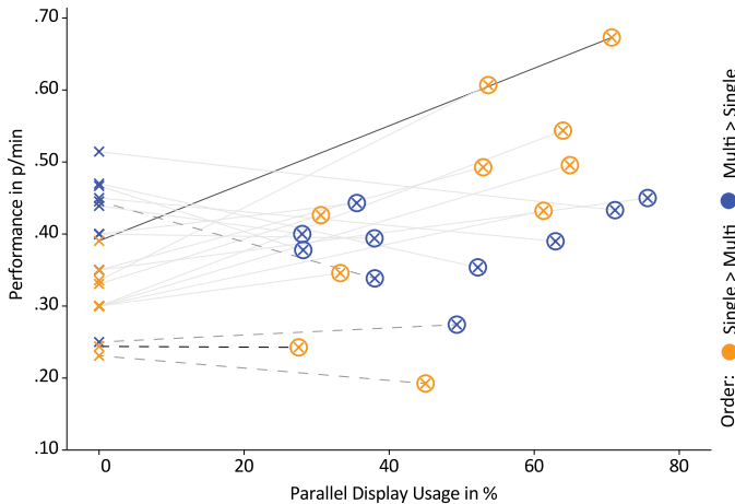
Fig. 12. Visual search performance of each participant pair with both display conditions (linked by grey lines) and plotted against the ratio of parallel display usage. The single-display condition (crosses) did not enable parallel display usage, while in the multi-display condition (encircled crosses), this possibility was exploited to different degrees. Learning effects between subsequent experiments depended on the order of conditions (color coded). The dotted lines represent the four groups, who knew each other only briefly. The exemplary groups 3 and 11 in Figure 11 are highlighted with a darker line between conditions.
