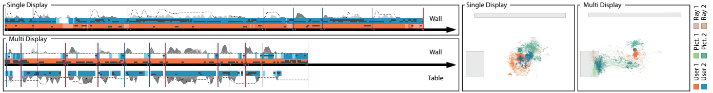
(a) Activity visualization of participant pair 3. In the single-display condition (upper timeline), the blue user primarily operated the handheld input devices, while the orange user was navigating. Eight perspectives were found. In the multi-display condition (lower timeline), a strategy of highly parallel display usage was applied. The blue user searched for perspectives at the tabletop display and joined her partner at the wall display in the final picture alignment phases. The group found the maximum number of 10 perspectives in less than 15 min.
